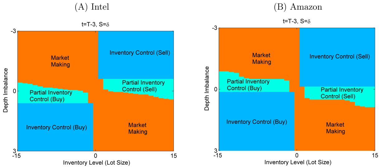
Figure 5: Optimal Strategy, spread = \delta , t = T - 3 , INTC (left) v.s. AMZN (right)
