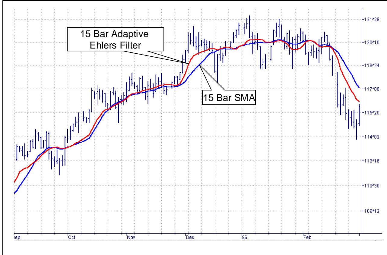
Figure 4. Performance of an Adaptive 15 Bar Ehlers Filter Compared to the Performance of a 15 Bar SMA
